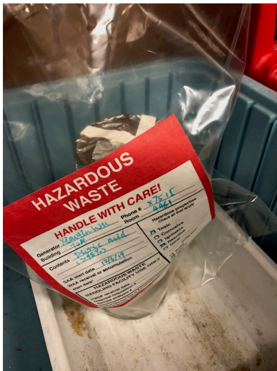
PICRIC ACID
